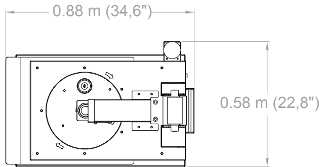
CAN COILER DIAM 360
