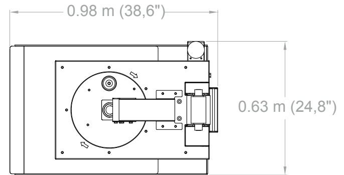
CAN COILER DIAM 500
